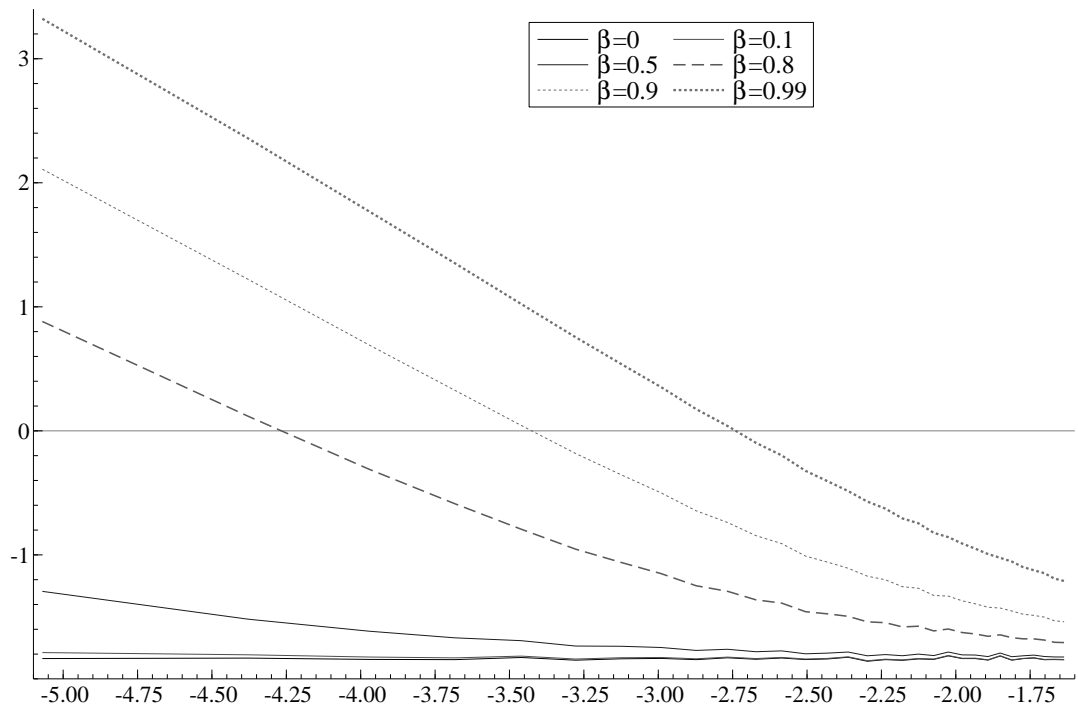
Figure 1: Monte Carlo averages over 10,000 replications of the log periodogram against the log of the first \sqrt{T} Fourier frequencies with T = 1,000 observations. The model is y_t = \beta y_{t+1}^e + x_t , x_t \stackrel{i.i.d.}{\sim} \mathbf{N}(0, 1) , and y_{t+1}^e is determined by RLS.
