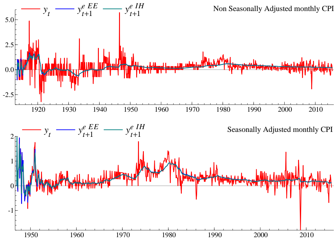
Figure 2: The figure report series of the U.S. monthly CPI inflation y_t together with its expectations under Euler-Equation (EE) and Infinite-Horizon (IH) learning, computed for the values of the forgetting factor \theta reported in Table 2. The top graph reports results for the non-seasonally adjusted series over 1913(2)-2015(8) and the bottom graph reports the seasonally adjusted series over 1947(1)-2015(8).
